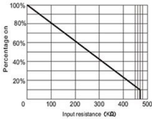
PERCENTAGE ON vs. INPUT RESISTANCE
