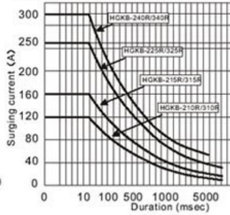
MAX. SURGE vs. DURATION
